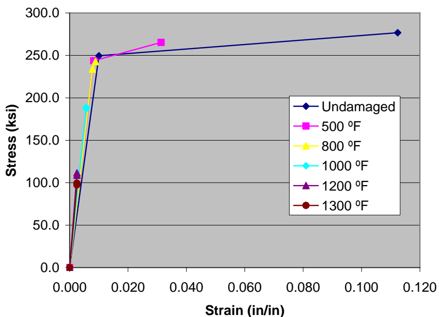
Figure 4.13 Stress vs. strain for 0.5 in. specimens of Phase I
