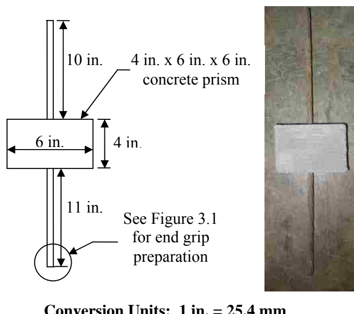
Figure 3.2 Schematic and actual view of pullout specimen
