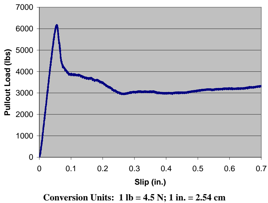
Figure 4.20 Pullout load vs. slip for a typical ductile failure (Specimen 11-1-1-2)
