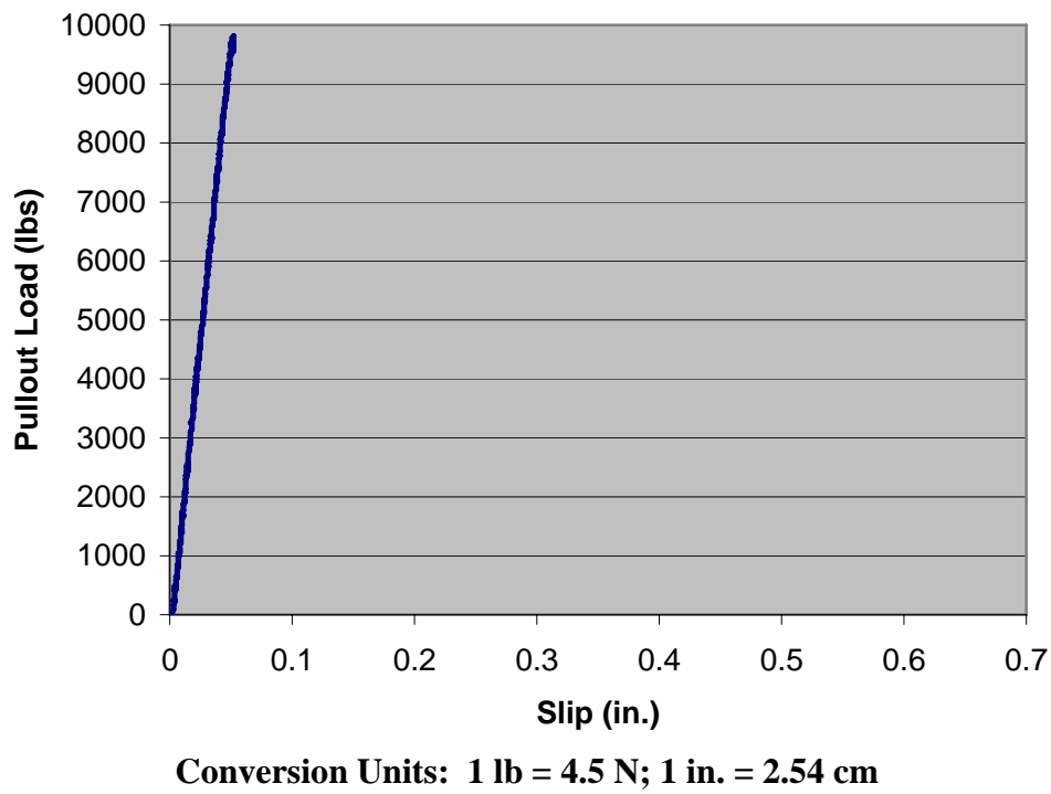
Figure 4.19 Pullout load vs. slip for a typical brittle failure (Specimen 14-2-1-2)
