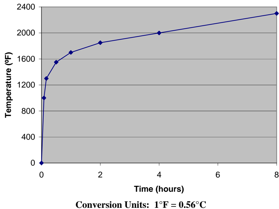
Figure 2.5 ASTM E 119-08 Standard Time-Temperature Curve
