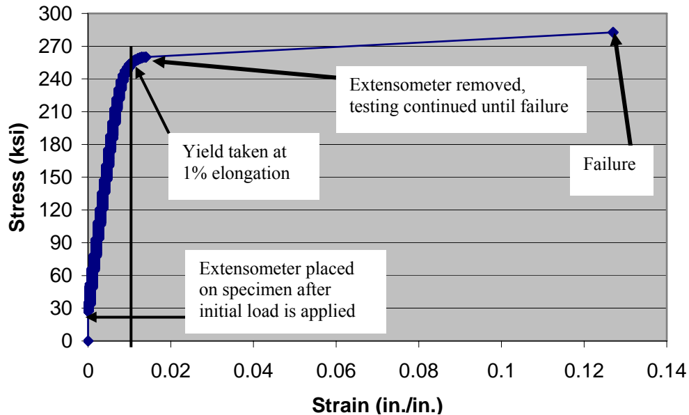
Figure 4.6 Typical stress-strain curve for tension testing
